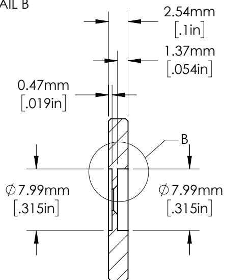
DETAIL B
