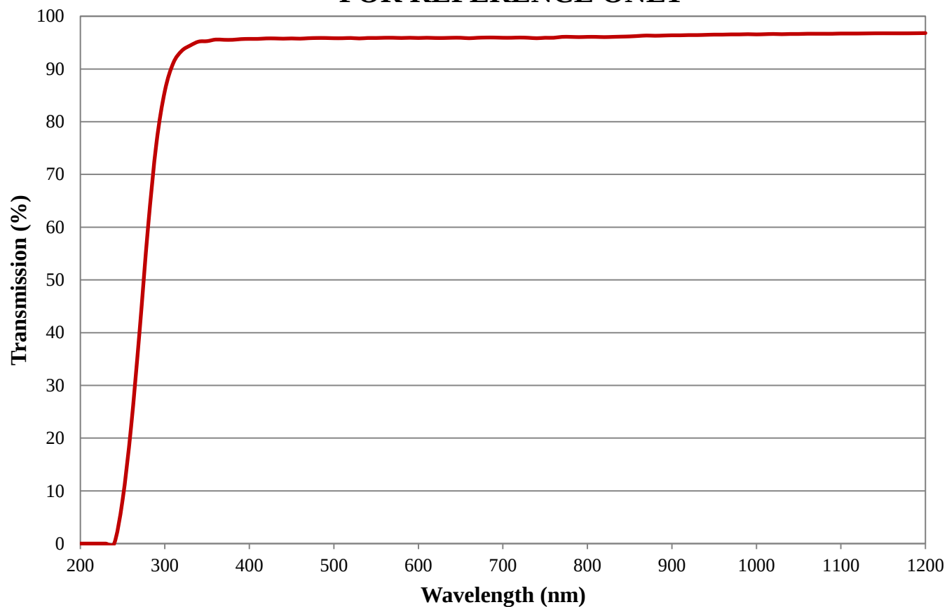
Hoya UV28N (280nm) Colored Glass Longpass Filter, 1mm Thickness Theoretical Transmission FOR REFERENCE ONLY
