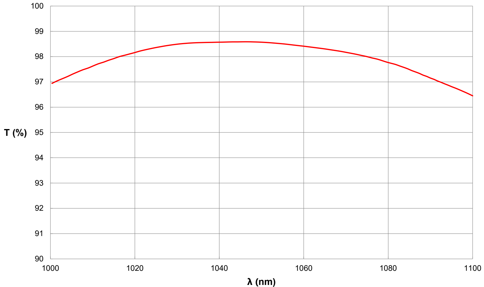
1064nm HP Flat Top Beam Shaper | \pi Shaper 12_12_1064_HP_W FOR REFERENCE ONLY
