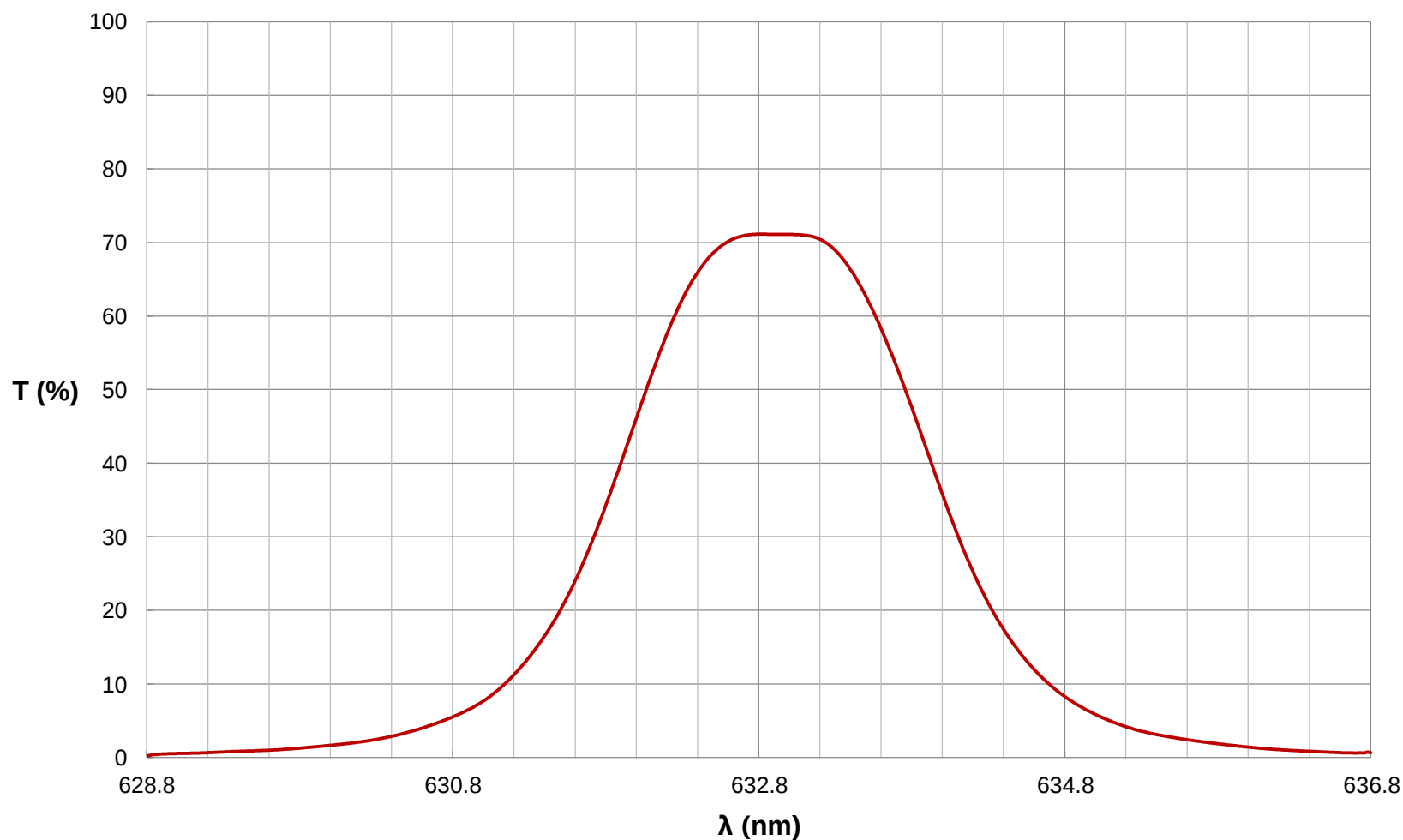
Ultra Narrow Traditional Coated Bandpass Filter, 632.8nm, 2.00 FWHM FOR REFERENCE ONLY
