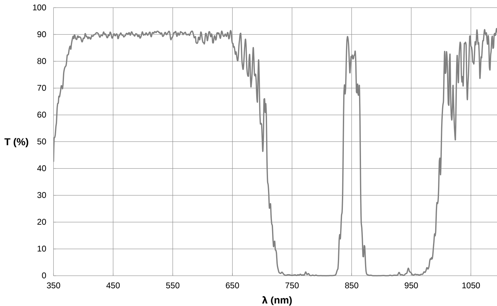
Everix Ultra-Thin Bandpass Filter, 850nm, OD 2.0 FOR REFERENCE ONLY
