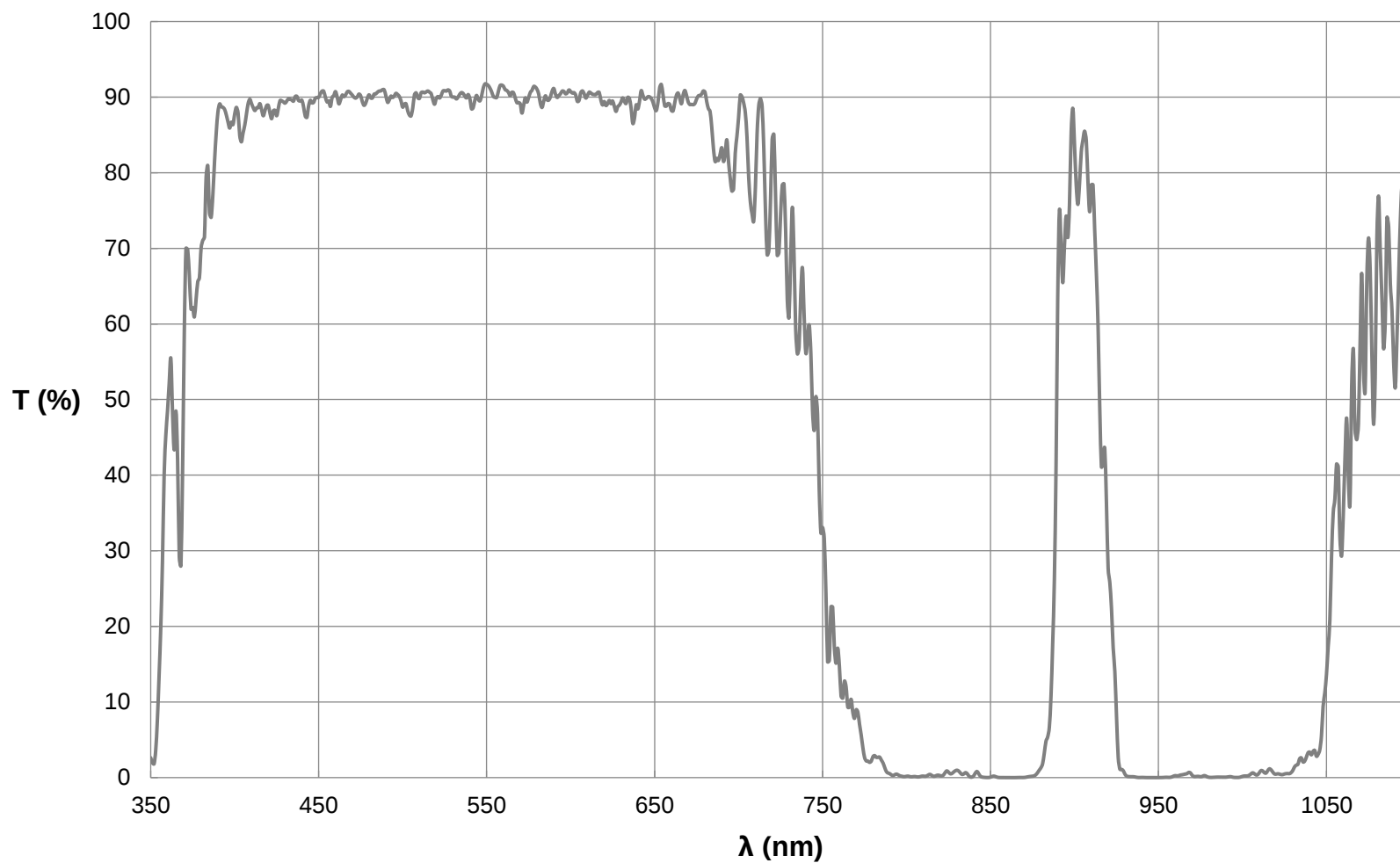
Everix Ultra-Thin Bandpass Filter, 905nm, OD 2.0 FOR REFERENCE ONLY
