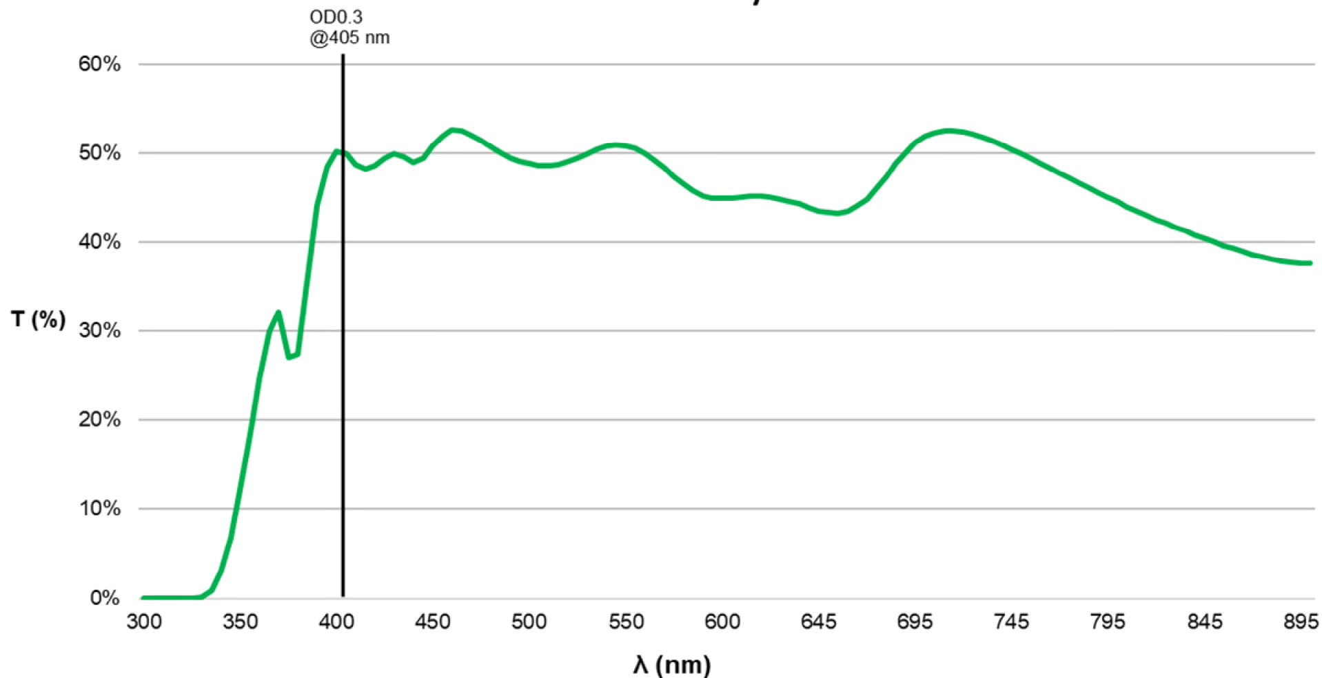
SCHOTT NG11 405 nm 50 Sq., 0.3 OD ND Filter REFERENCE Only
