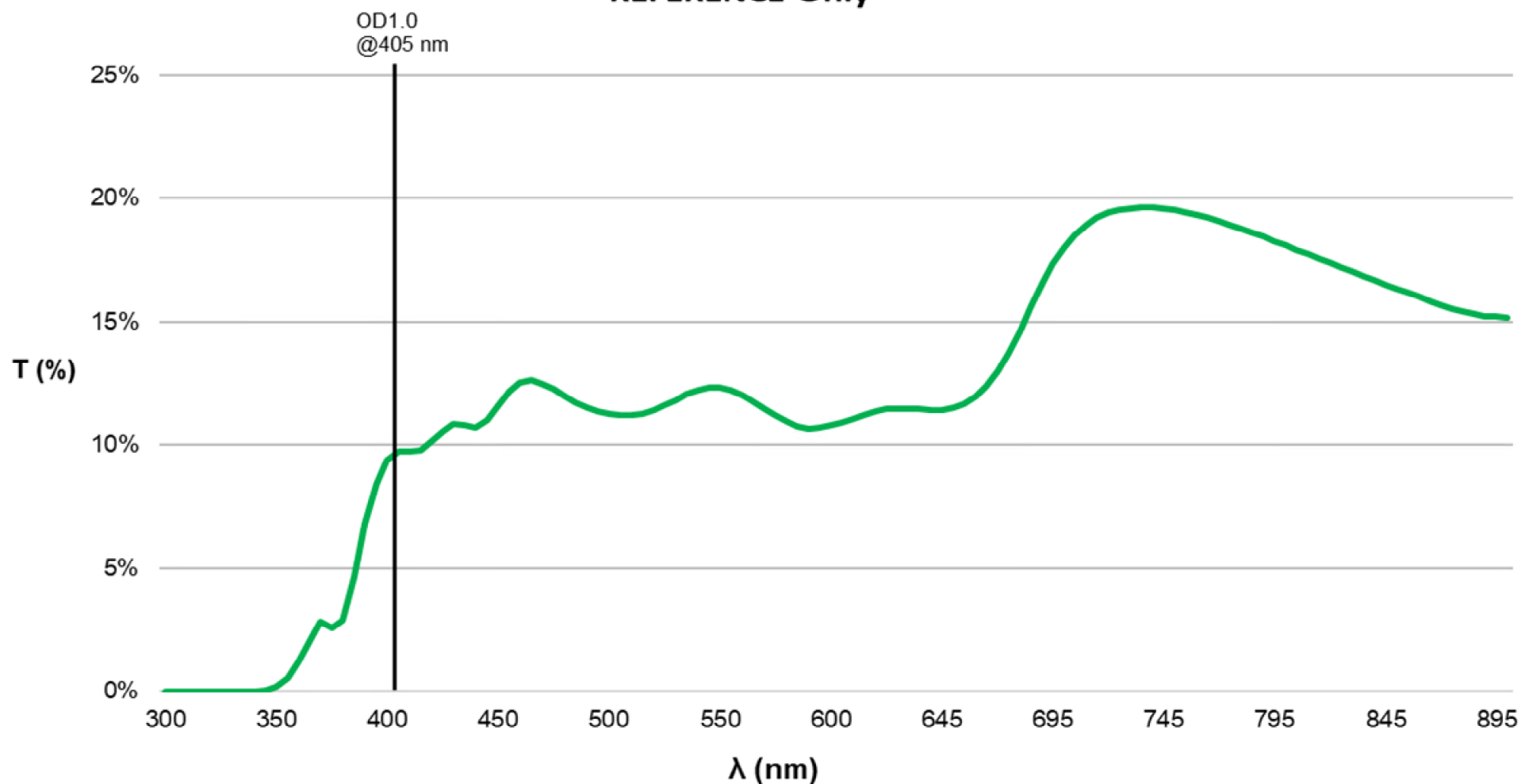
SCHOTT NG4 405 nm 50 Sq., 1.0 OD ND Filter REFERENCE Only
