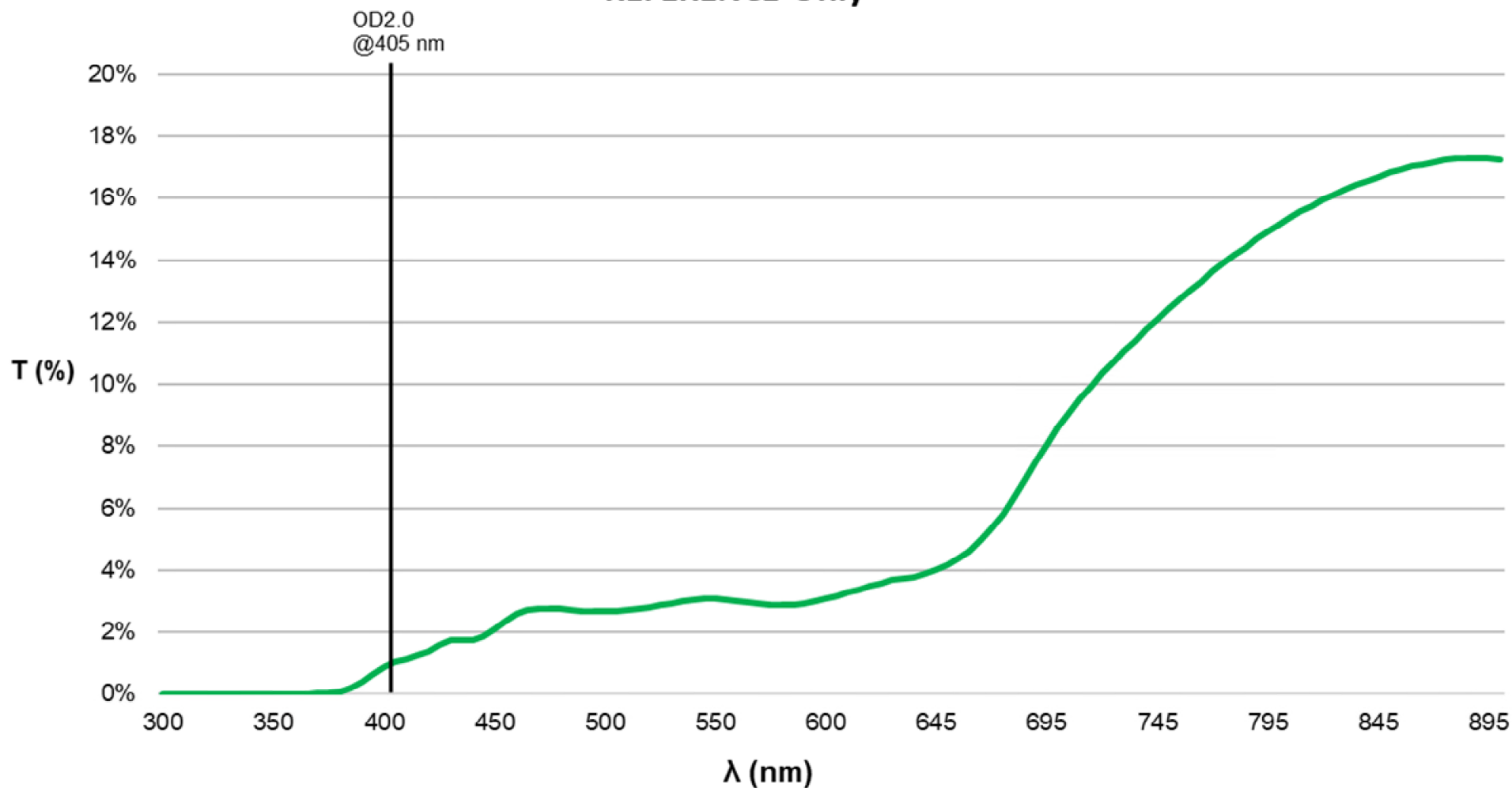
SCHOTT NG3 405 nm 50 Sq., 2.0 OD ND Filter REFERENCE Only
