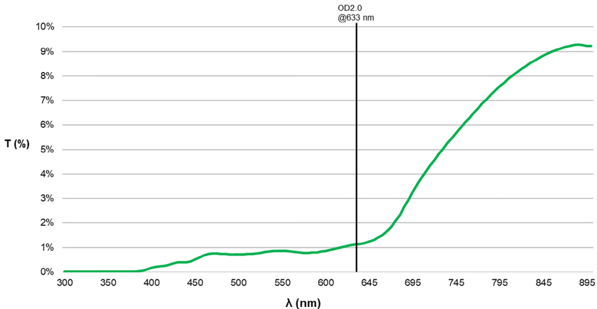
SCHOTT NG3 633 nm 50 Sq., 2.0 OD ND Filter REFERENCE Only
