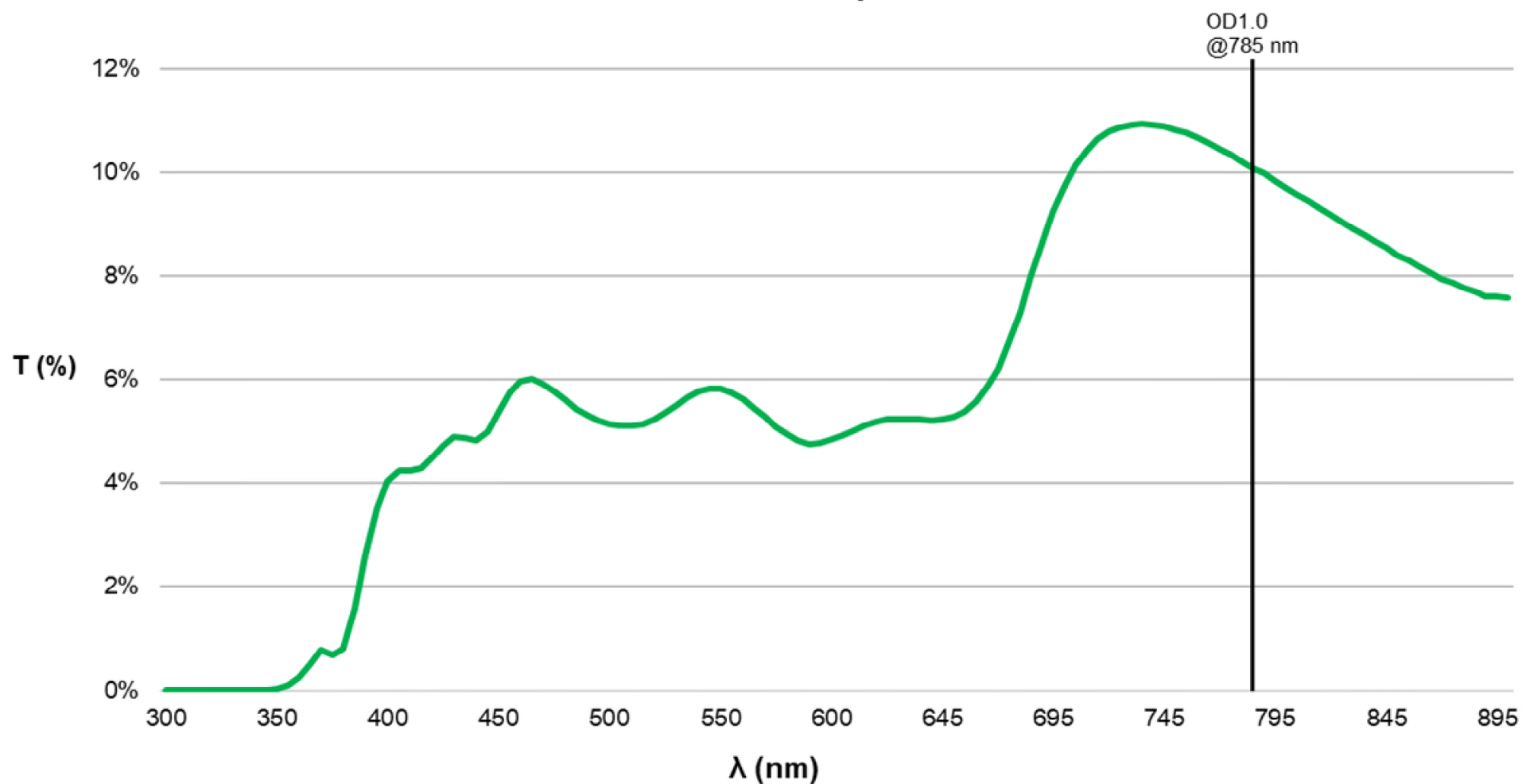
SCHOTT NG4 785 nm 50 Sq., 1.0 OD ND Filter REFERENCE Only
