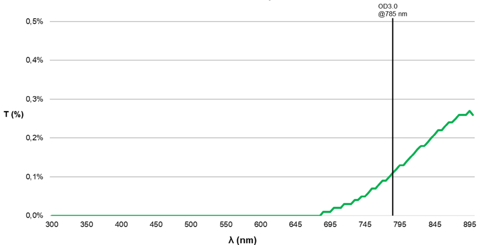
SCHOTT NG1 785 nm 50 Sq., 3.0 OD ND Filter REFERENCE Only
