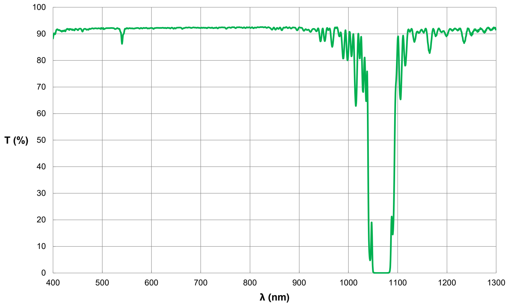
Everix Ultra-Thin OD 4 Notch Filter, 1064nm, 12.5mm Diameter FOR REFERENCE ONLY
