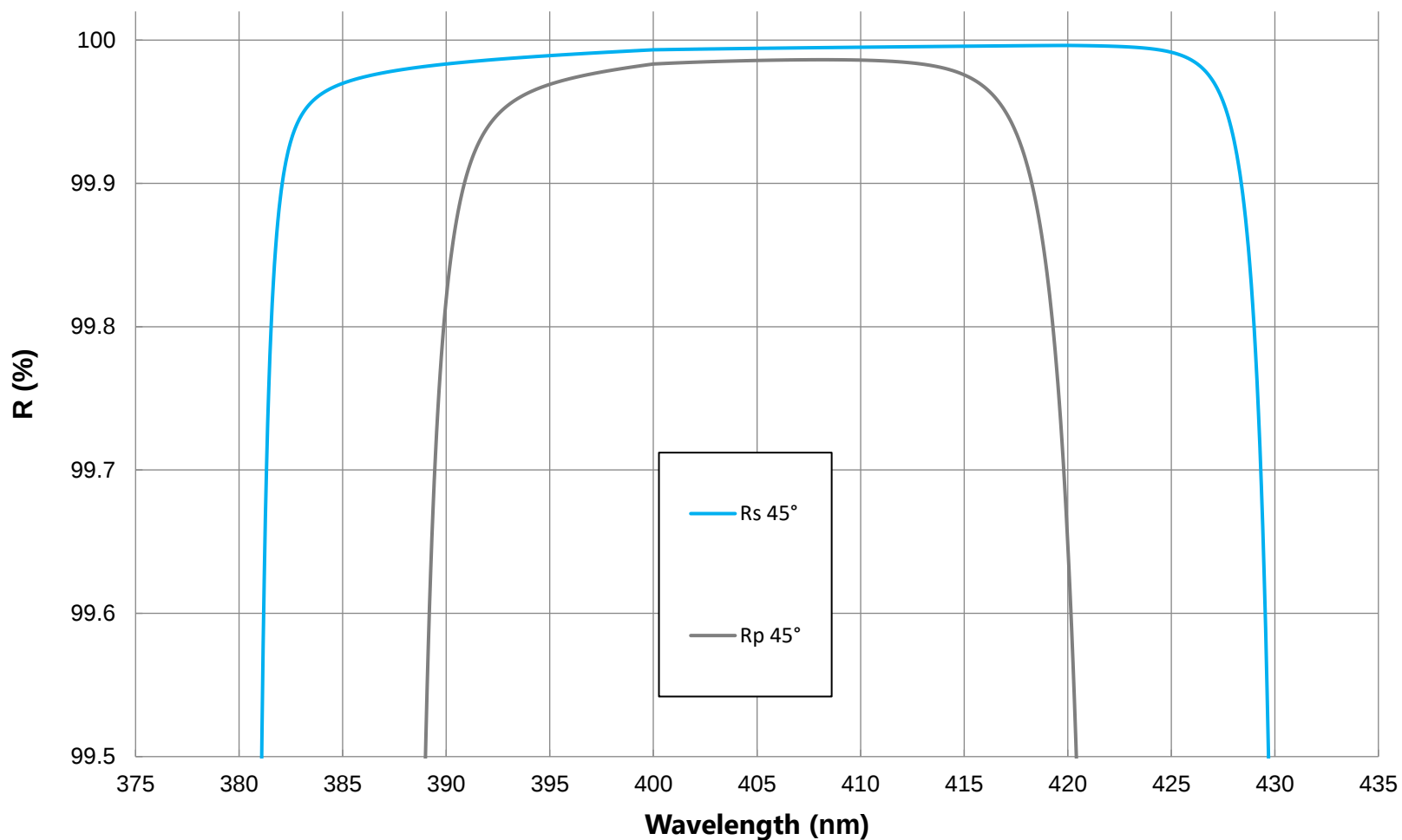
385 - 415nm Reflectance FOR REFERENCE ONLY
