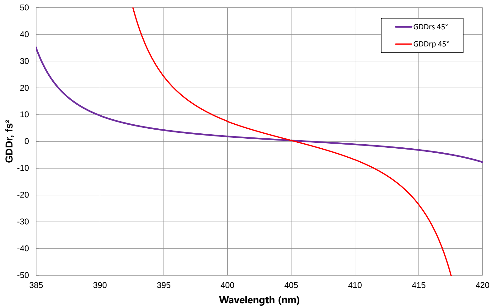
385-415nm GDD Performance FOR REFERENCE ONLY
