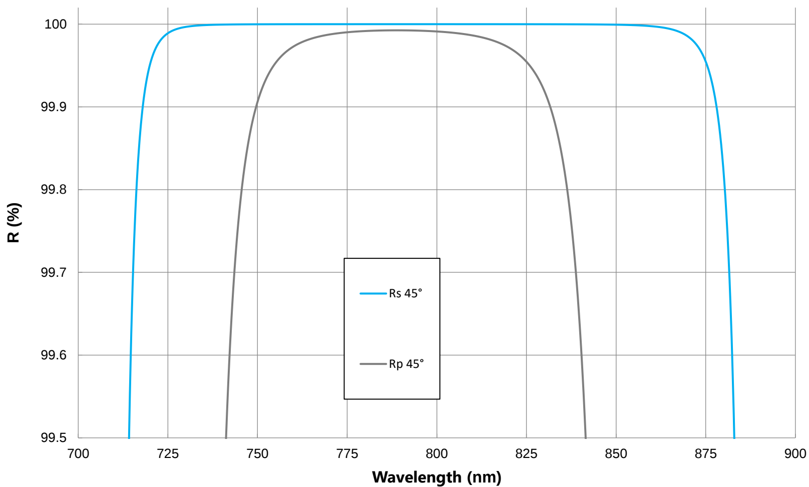
770 - 830nm Reflectance FOR REFERENCE ONLY
