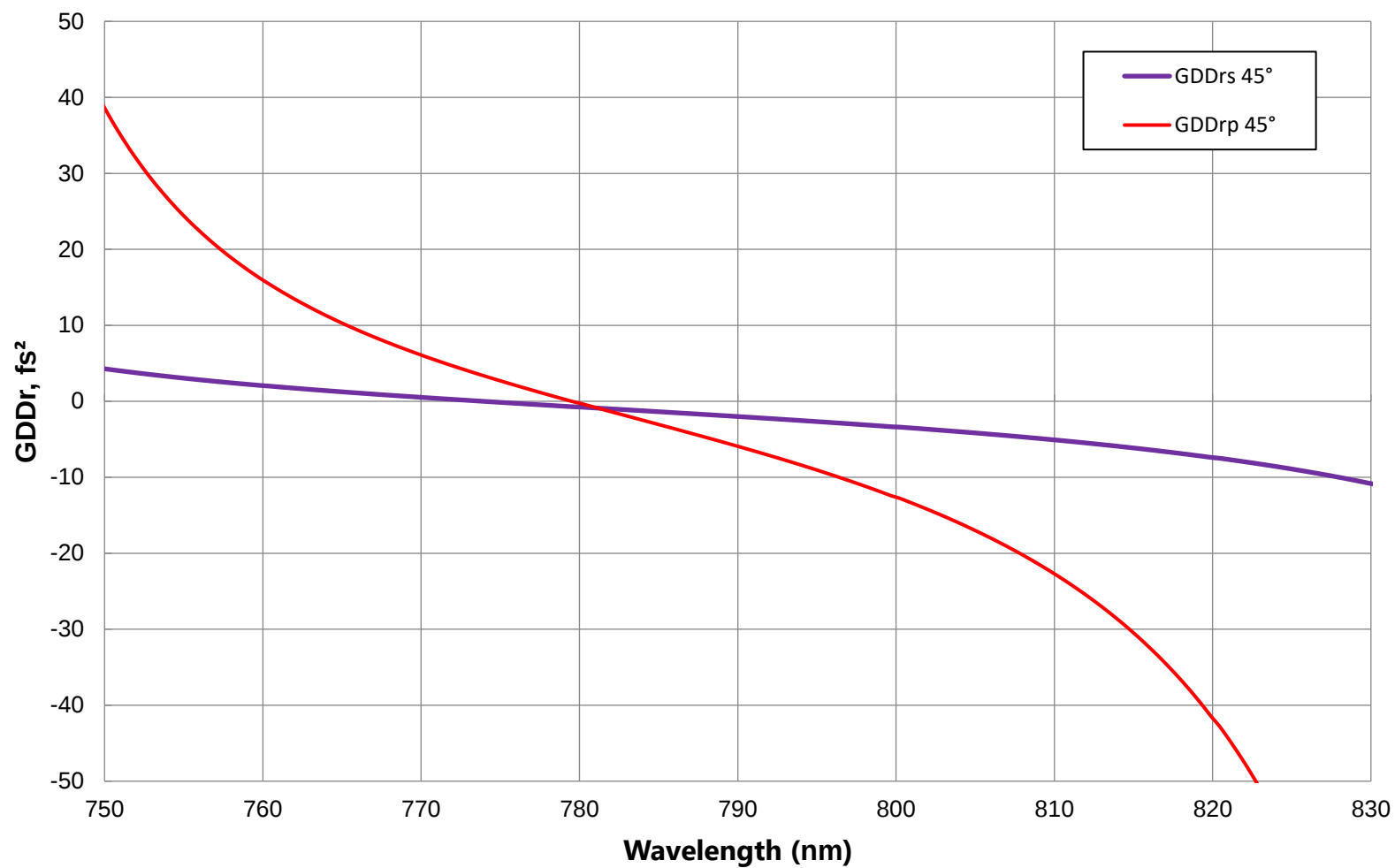
770 - 830nm GDD Performance FOR REFERENCE ONLY
